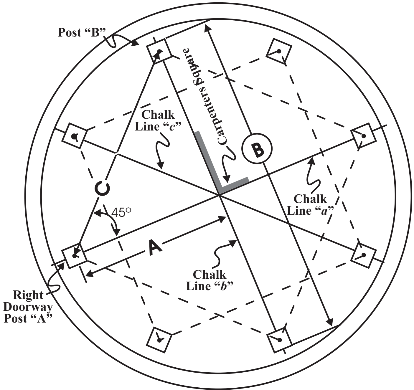
Fig. 1 Tiffany Gazebos Post Layout
